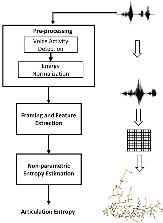
Fig. 1. Framework for calculating articulation entropy.
